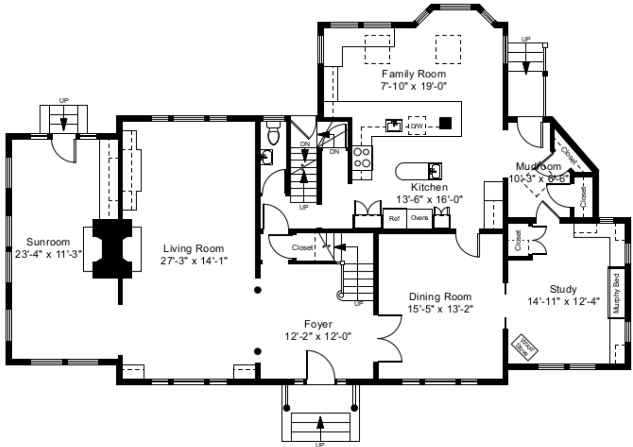
First Floor Plan Ceiling Height = 8'-4"
