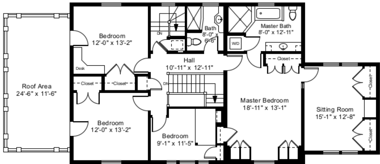
Second Floor Plan Ceiling Height = 8'-0"
